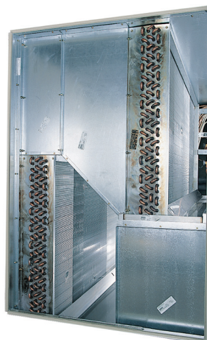
Figure 5: Extended Face Area Coils
