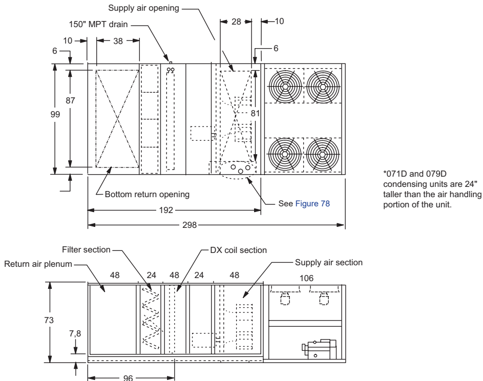
Figure 75: RDT 070D to 079D
