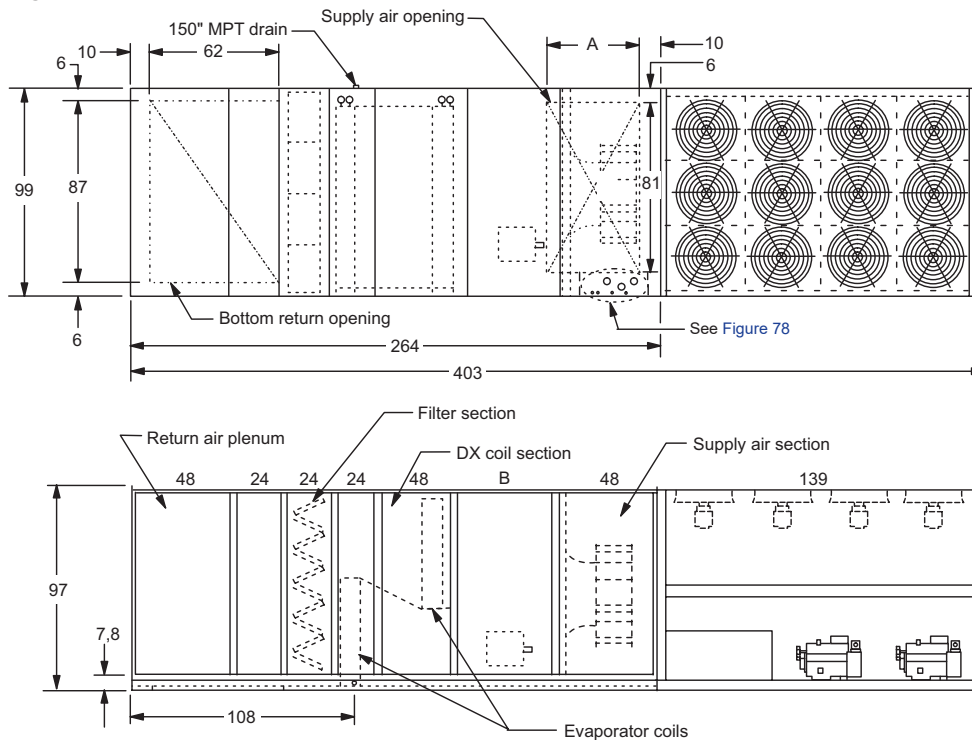
Figure 76: RDT 080D to 140D
