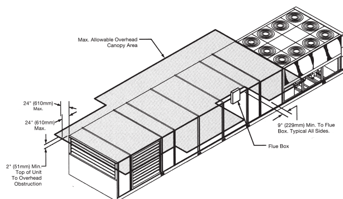
Figure 97: Ventilation Clearances
