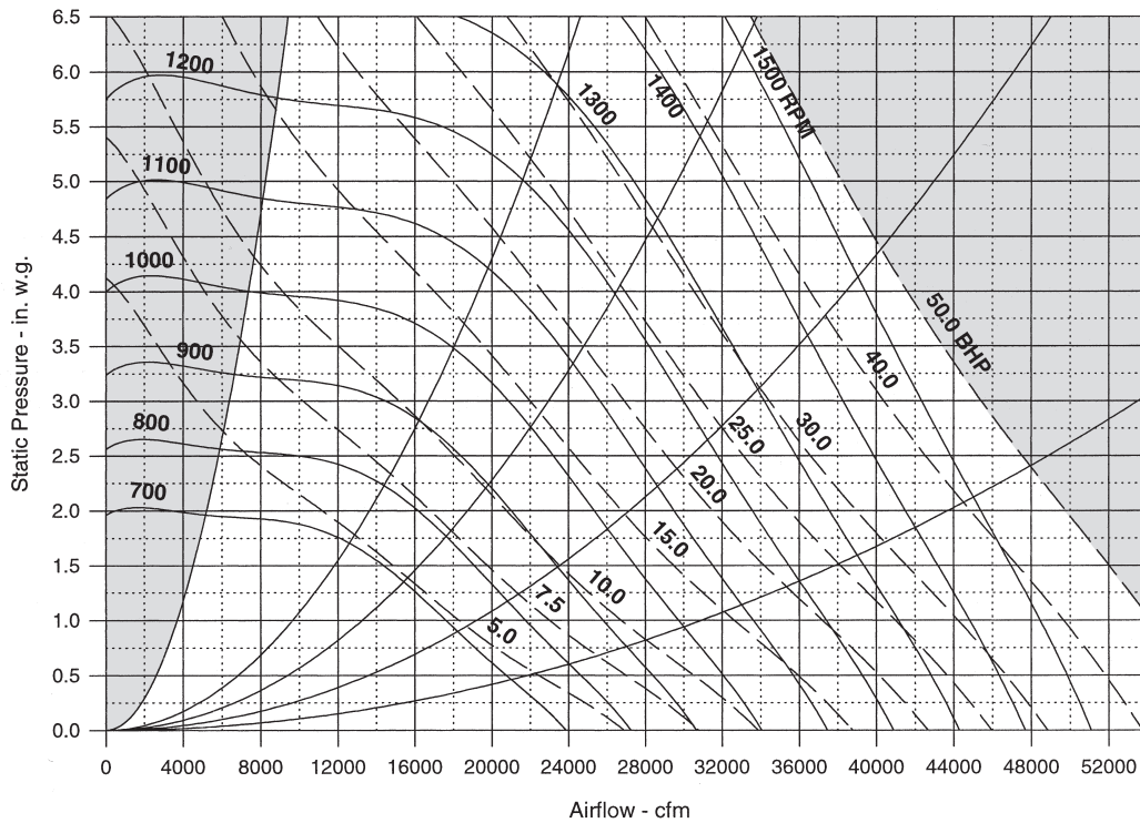
Figure 57: RPS/RFS 080D to 105D 33 in. Airfoil Supply Fan
