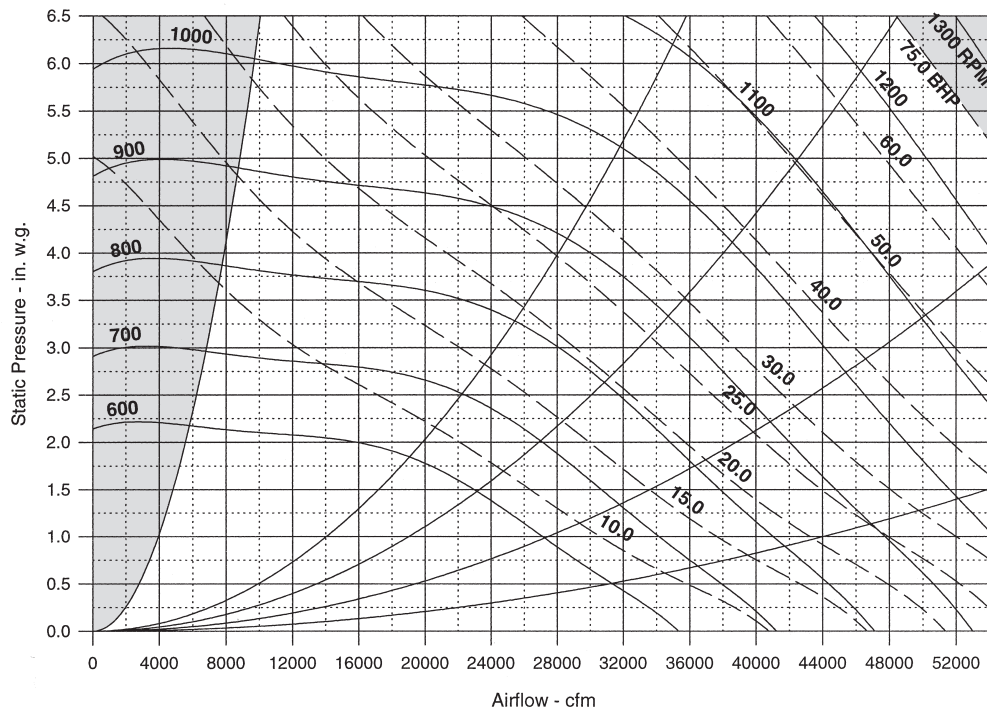
Figure 59: RPS/RFS 080D to 140D 40 in. Airfoil Supply Fan
