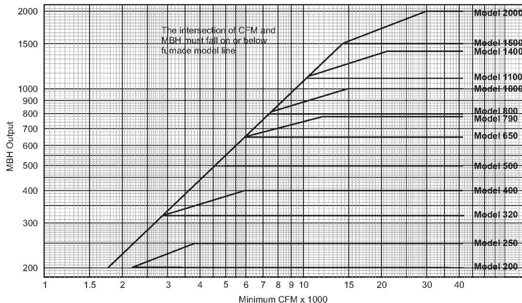
Figure 37: Gas Heat Capacity
