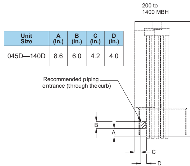
Figure 80: 200 to 1400 MBh Gas Heat/Heat Section
