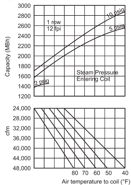
Figure 46: Steam Coil, Medium Capacity, 080D to 140D
