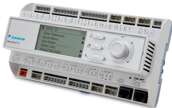
Figure 23: MicroTech Keypad/Display
