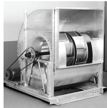
Figure 11: SWSI Airfoil Fans (RDT)
