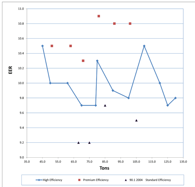
Figure 2: EER Options
