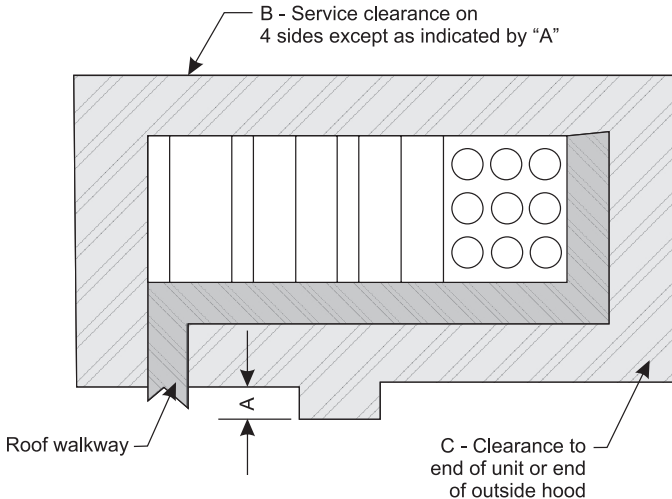
Figure 96: Service Clearances
