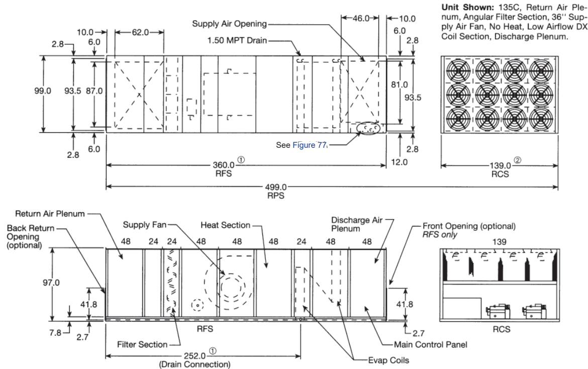
Figure 73: RPS/RFS/RCS 110D to 140D
