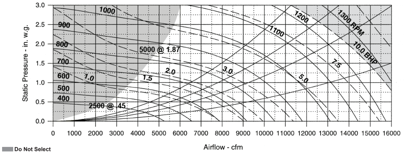
Figure 64: RPS/RFS/RDT 080D to 140D, 44 in. SWSI Airfoil Return Fan
