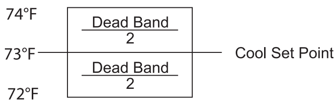
Figure 28: Compressorized Logic
